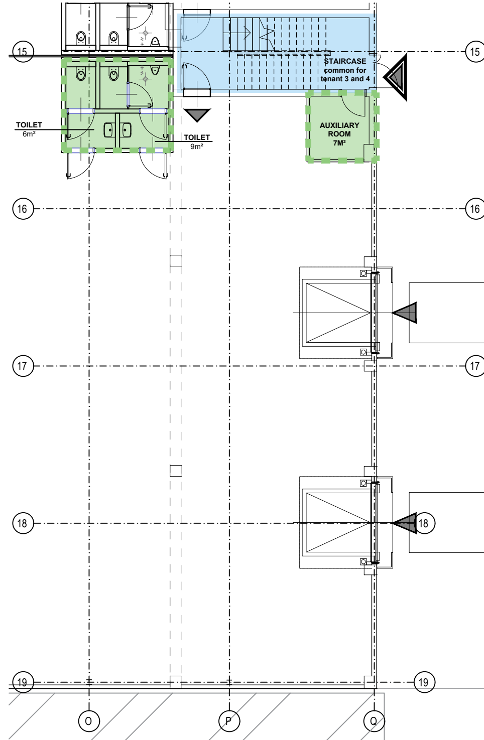
GROUND FLOOR
