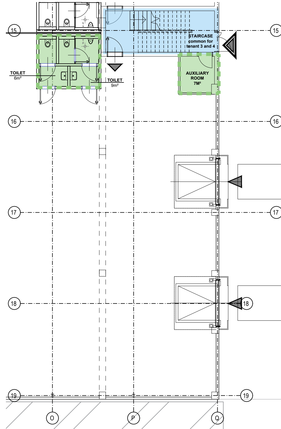
GROUND FLOOR
